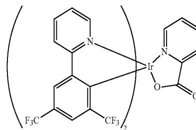
bis-{2-[3,5-bis(trifluoromethyl)phenyl]pyridinato-N,C2'} iridium(III)-picolinate [Ir(CF 3 ppy) 2 (Pic)]
