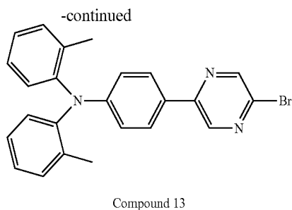
N-(4-(5-bromopyrazin-2-yl)phenyl)-2-methyl-N-(o-tolyl)aniline (Compound 13)
