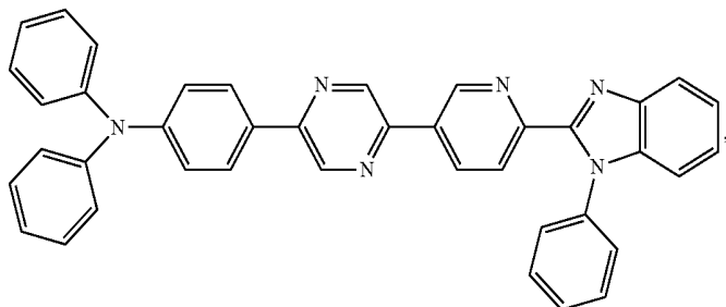
N,N-diphenyl-4-(5-(6-(1-phenyl-1H-benzo[d]imidazol-2-yl)pyridin-3-yl)pyrazin-2-yl)aniline
