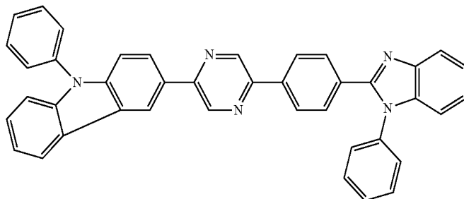
9-phenyl-3-(5-(4-(1-phenyl-1H-benzo[d]imidazol-2-yl)phenyl)pyrazin-2-yl)-9H-carbazole
