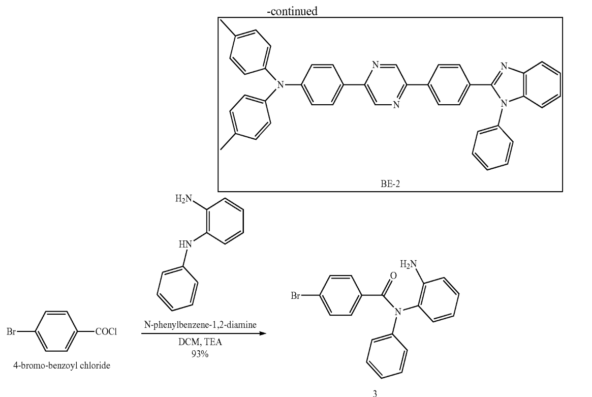
4-Bromo-N-(2-(phenylamino)phenyl)benzamide (Compound 3)
