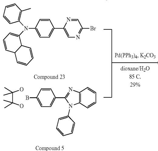
Compound 23
