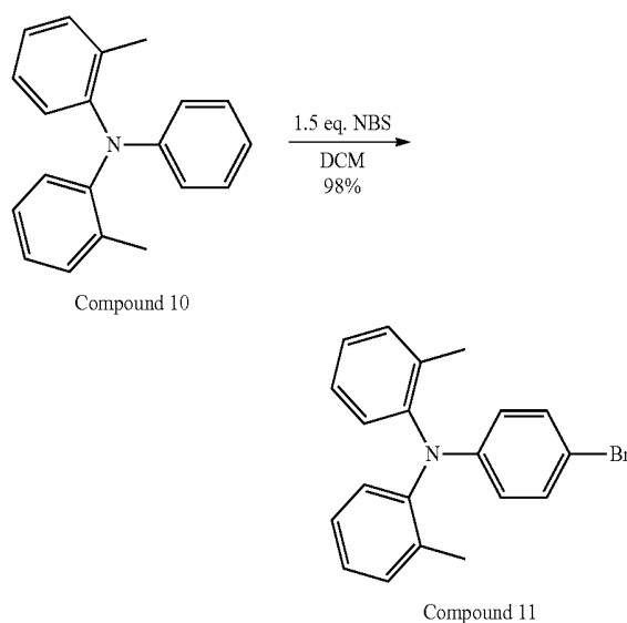
N-(4-bromophenyl)-2-methyl-N-(o-tolyl)aniline (Compound 11)
