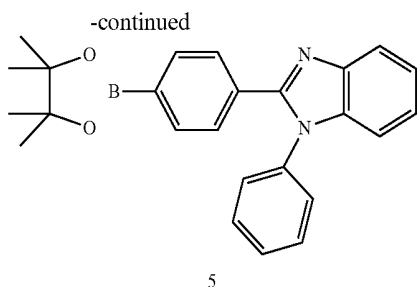
1-phenyl-2-(4-(4,4,5,5-tetramethyl-1,3,2-dioxaborolan-2-yl)phenyl)-1H-benzimidazole (5)
