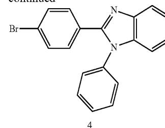
2-(4-bromophenyl)-1-phenyl-1H-benzo[d]imidazole (4)
