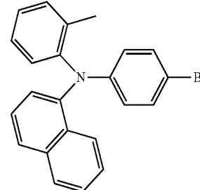
Compound 21
