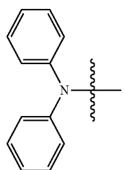
unsubstituted diphenylamine
