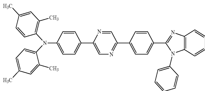
N-(2,4-dimethylphenyl)-2,4-dimethyl-N-(4-(5-(4-(1-phenyl-1H-benzo[d]imidazol-2-yl)phenyl)pyrazin-2-yl)phenyl)aniline
