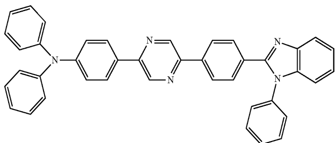
N,N-diphenyl-4-(5-(4-(1-phenyl-1H-benzo[d]imidazol-2-yl)phenyl)pyrazin-2-yl)aniline
