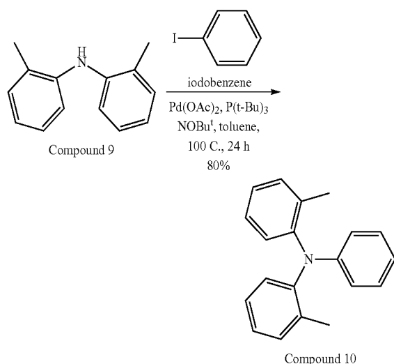
2-methyl-N-phenyl-N-(o-tolyl)aniline (Compound 10)
