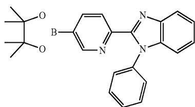
Compound 2
