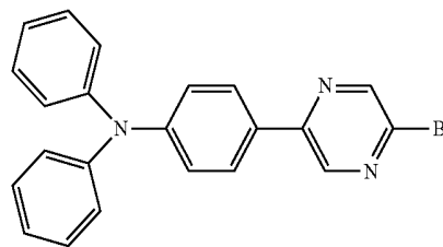
Compound 19
