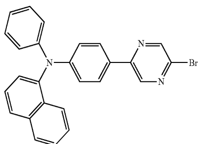
Compound 8
