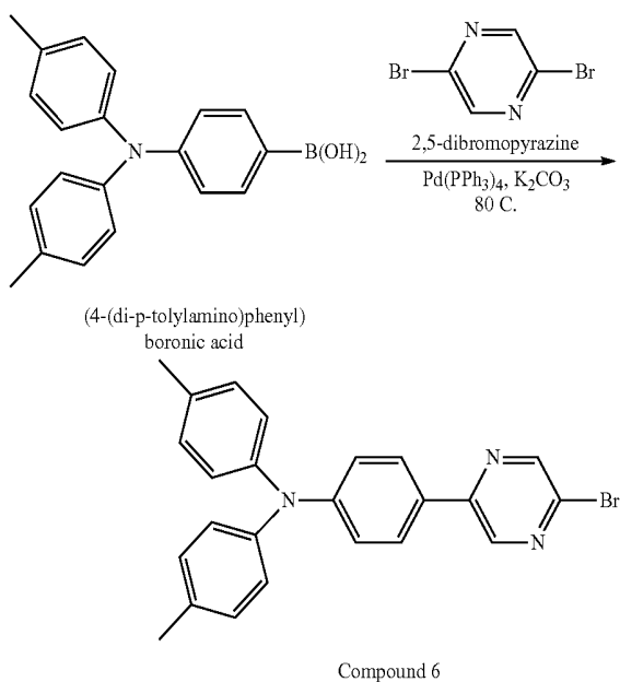
4-(5-bromopyrazin-2-yl)-N,N-di-p-tolylaniline (Compound 6)
