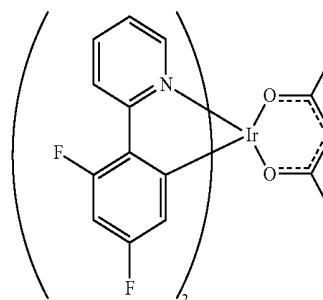
bis(2-[4,6-difluorophenyl]pyridinato-N,C2') iridium(III) (acetylacetonate) [Flr(acac)]
